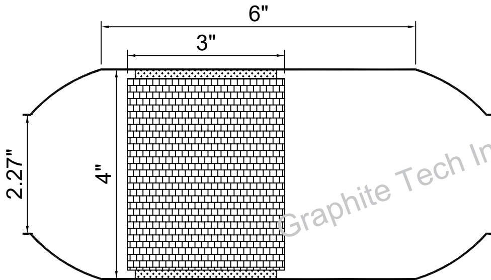
Part No : G4-2.25-6-3
