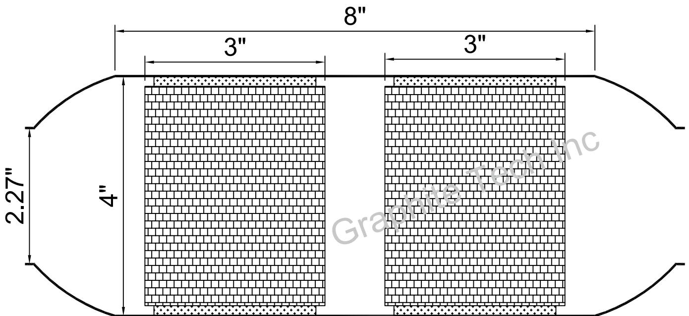
Part No : G4-2.25-8-3+3
