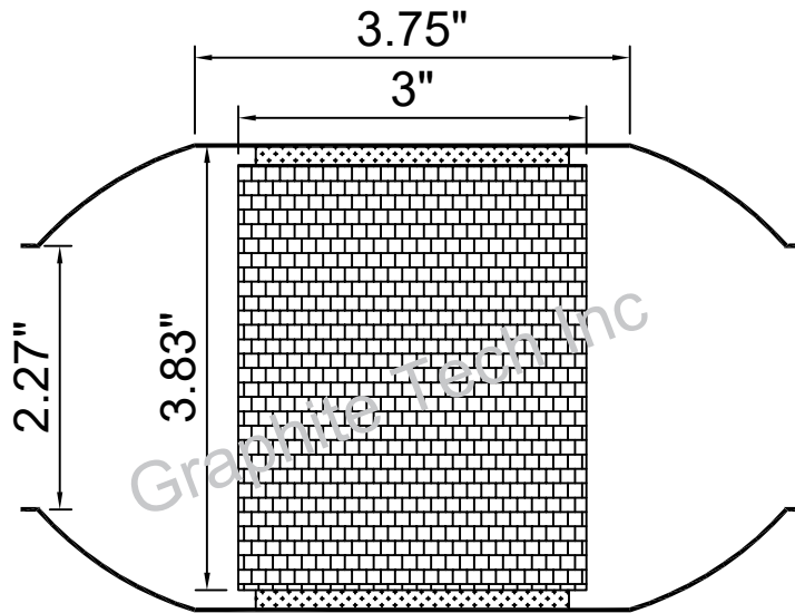
Part No : G4-2.25-3.75-3
