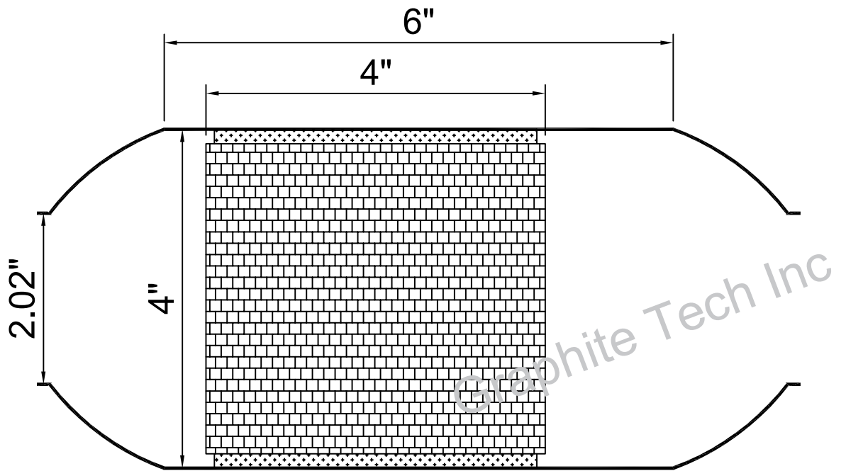
Part No : G4-2-6-4
