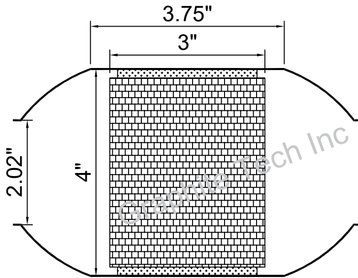
Part No : G4-2-3.75-3
