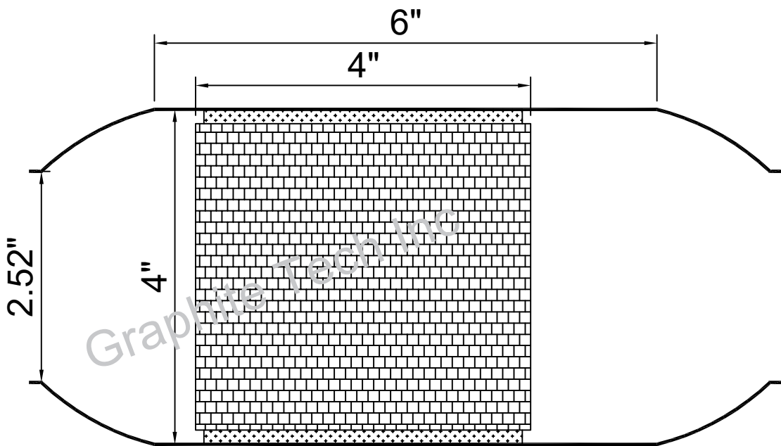
Part No : G4-2.5-6-4
