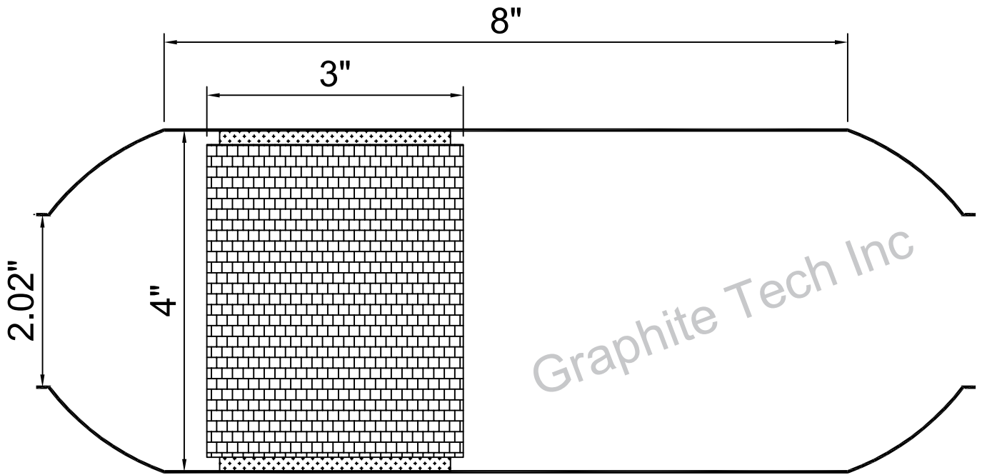
Part No : G4-2-8-3
