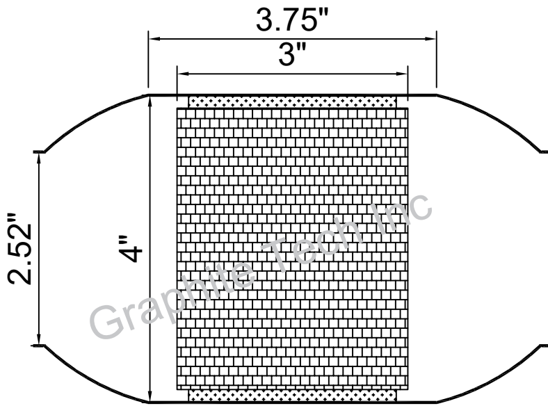
Part No : G4-2.50-3.75-3
