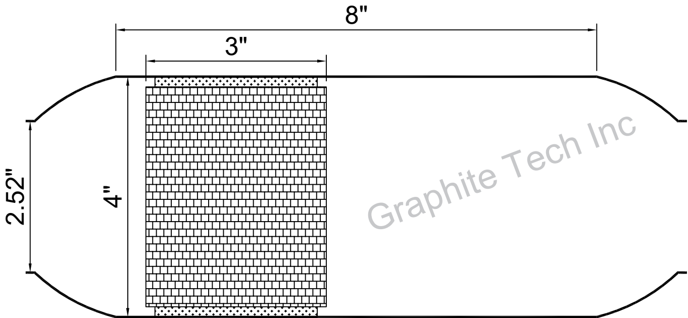
Part No : G4-2.5-8-3
