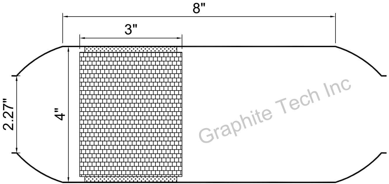
Part No : G4-2.25-8-3
