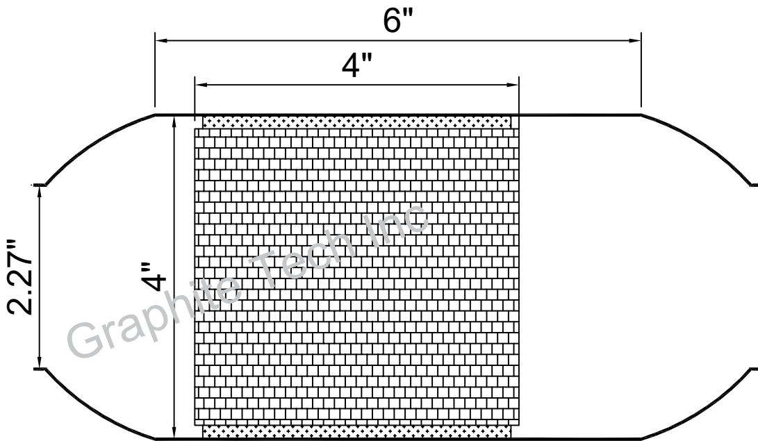
Part No : G4-2.25-6-4
