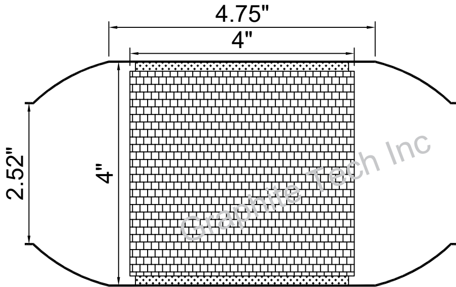
Part No : G4-2.50-4.75-3
